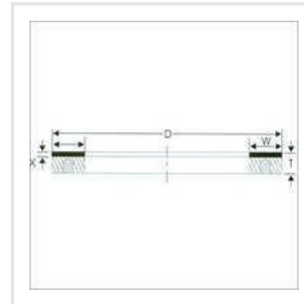
Cylinder Diamond In Rim
