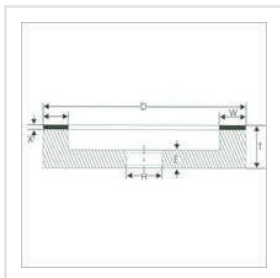
Plain Cup Diamond In Rim
